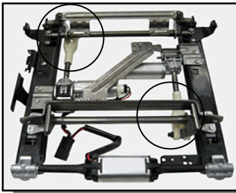
Seat Actuator Gearbox Thrust Bearings
